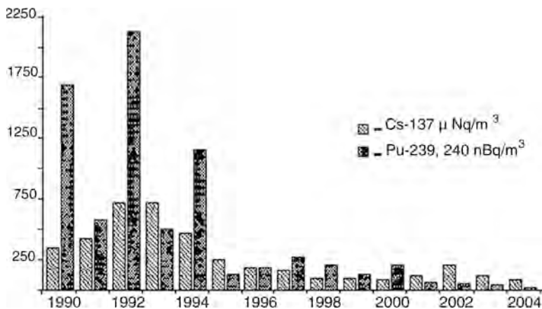
Figure 8.1. Dynamics of the radionuclides Pu-239, Pu-240, and Cs-137 in the surface air in Khoyniky, Belarus, 1990–2004 (Konoplya et al. , 2006).
