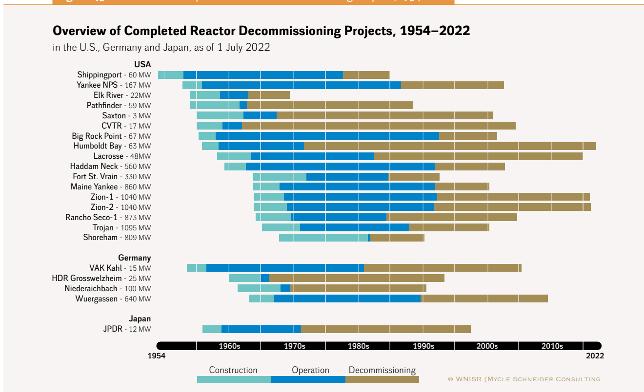
Figure 45 · Overview of Completed Reactor Decommissioning Projects, 1954–2022
