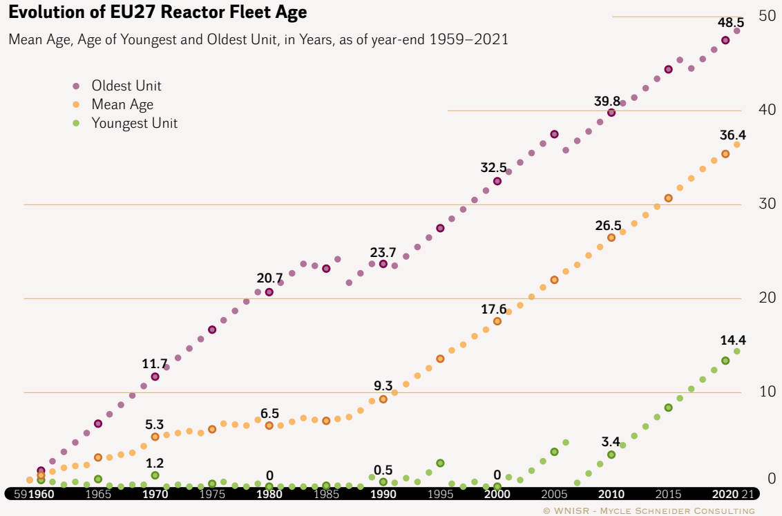
Figure 67 · Age Evolution of EU27 Reactor Fleet, 1959–2021
